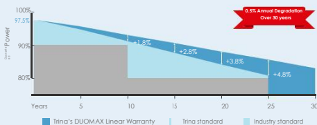
Trina Solar's DUOMAX Linear Performance Warranty
